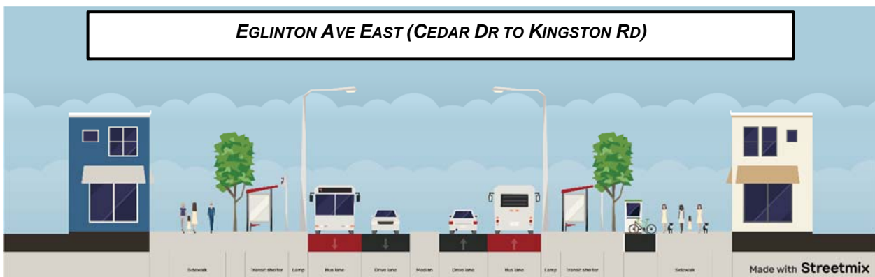
FIGURE 5: EGLINTON AVENUE EAST – 2 GENERAL PURPOSE LANE + 2 BUS LANE CROSS-SECTION
