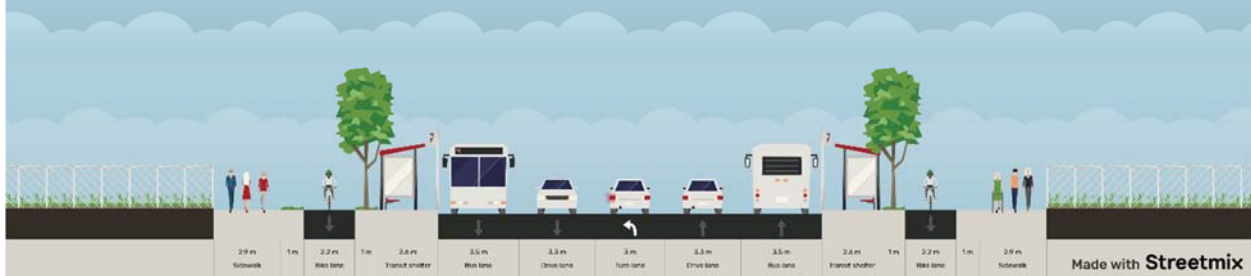
FIGURE 7: FINCH AVENUE EAST – CONCEPTUAL CROSS-SECTION FOR 36-METRE ROW
