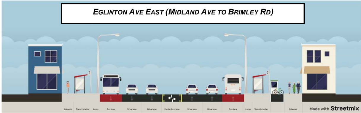
FIGURE 4. EGLINTON AVENUE EAST – 4 GENERAL PURPOSE LANE + 2 BUS LANE CROSS-SECTION
